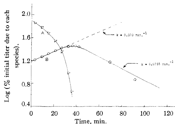
Fig. 4.—Change with time of concentration of \text{MnO}_4^- (A) and \text{Mn}(\text{C}_2\text{O}_4)_2^{2-} (B). Solution was mixed to contain 1.000 \times 10^{-4} M \text{KMnO}_4 , 0.50 \times 10^{-4} M \text{Mn}(\text{ClO}_4)_2 , 200 \times 10^{-4} M \text{Na}_2\text{C}_2\text{O}_4 , 20 \times 10^{-4} M \text{HClO}_4 and 1.00 M \text{NaClO}_4 .
