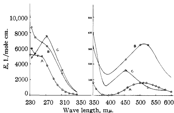
Fig. 1.—Molar extinction coefficients of manganese(III) complexes: A, \text{Mn}(\text{H}_2\text{P}_2\text{O}_7)_3^{\equiv} ; B, \text{Mn}(\text{C}_2\text{O}_4)_3^{\equiv} (cherry red); C, \text{Mn}(\text{C}_2\text{O}_4)_2^- (yellow).
